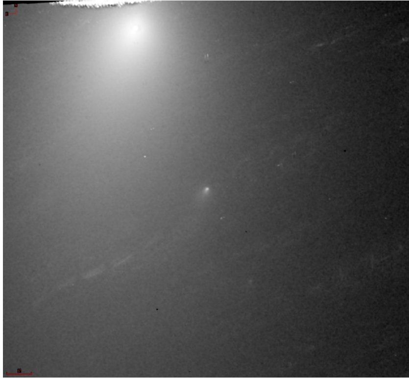
Fig 1. HST image showing the new discovered cometary object close to the main nucleus of comet C/2017 O1. Stack of four images taken on Dec. 01, 2017 with filter F110W by HST.
