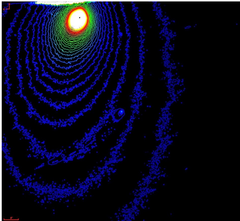
Fig. 2. Same image shown in color isophotes to highlight the extent of the coma of the two bodies.
