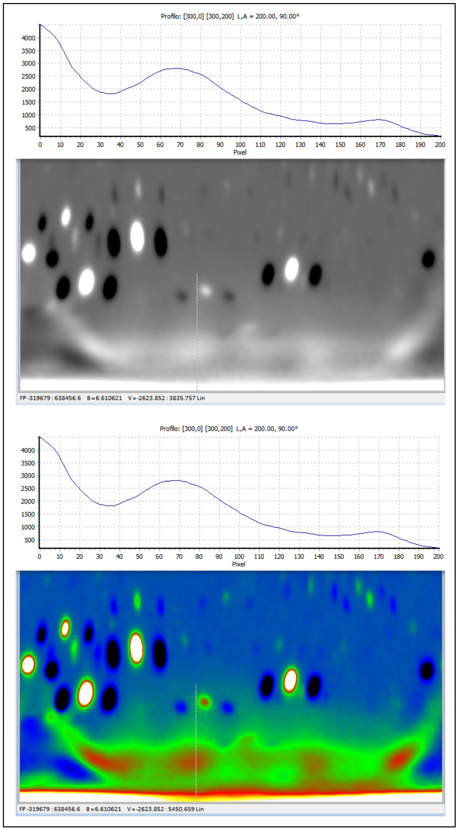
Figure 1 An example of the polar transformation of the image and of the photometric profile drawn at PA 150° is shown with two different visualization methods. Details on the processing procedure are given in the text. Image taken at LCO-Haleakala Observatory on July 28, 2023.
