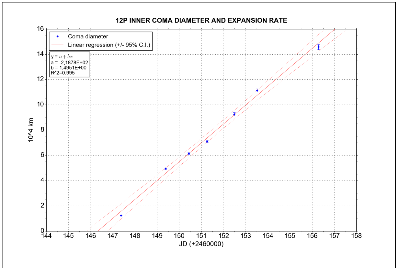
Figure 2 The measurements ( \pm SD) of the diameters of the coma are indicated by the blue diamonds. The red solid line is the linear regression (dotted lines=C.I. 95%). The slope indicates the expansion rate of the inner coma of comet 12P after a possible second outburst.
